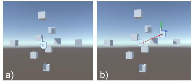
Figure 5: Design of Dynamic Coordinate Line(s) (DCL) boundary awareness method. (a) The coordinate lines are not shown if they are 1.5cm away from the interaction boundary. (b) When users are about to move outside the interaction volume, at 1.5cm to the boundary, DCL would highlight the corresponding coordinate line(s) to let users be aware that they may possibly be exiting the area.
